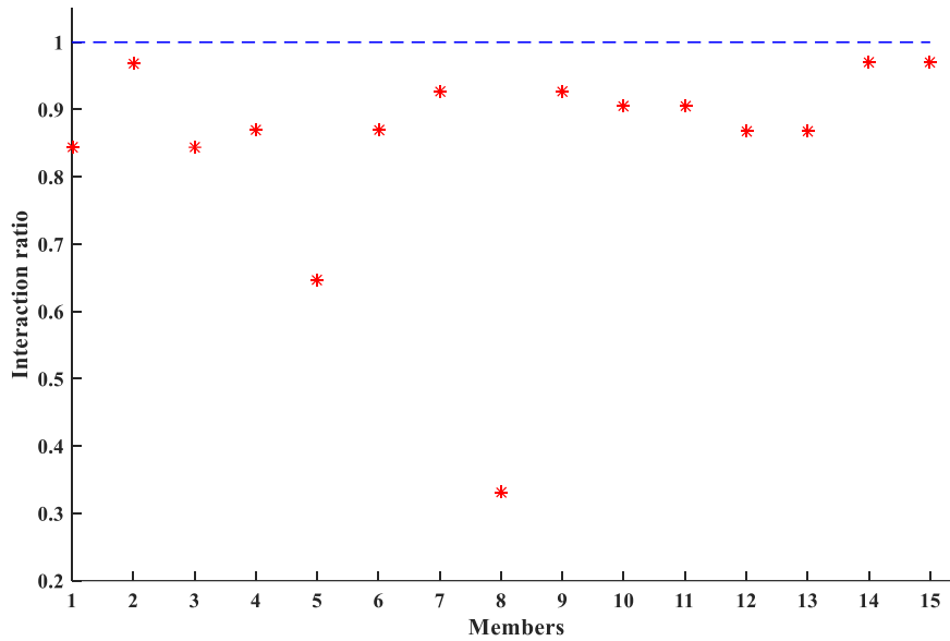
Figure 9. Members strength interaction ratio of 2x3 frame
