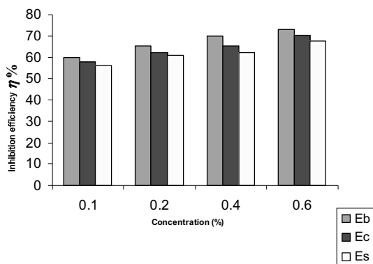
Fig. 2. Variation of inhibition efficiency with concentration of stem extract for Tin in 3.0 M \text{HNO}_3
