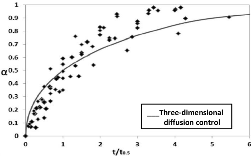
Fig. 11. Plot of \alpha vs. t/t_{0.5} for diffusion rate-controlling situation.
