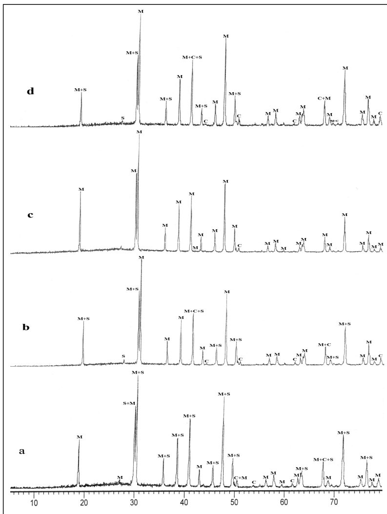
Fig. 6a-d. XRD patterns of 38 \mu m particle size of kyanite sintered at different temperatures during soaking time constant of 2 hours a: 1400 ^{\circ} C b: 1500 ^{\circ} C c: 1550 ^{\circ} C and d: 300 \mu m - 1550 ^{\circ} C /2 h M: Mullite Sil: Silimanite Crn: Corundum [16]
