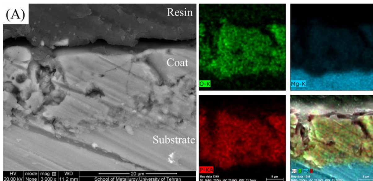
Fig. 3. Cross section SEM micrographs and elemental distribution map of a) P-coating, b) Si-coating, c) Al-coating.
