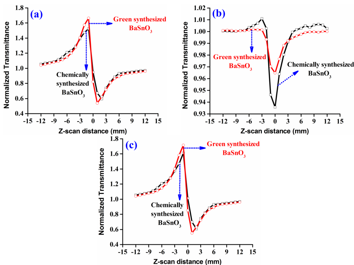
Fig. 11. Z-scan plots of CBS and GBS
