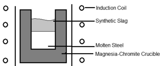
Fig. 2. Schematic diagram of experimental apparatus.
