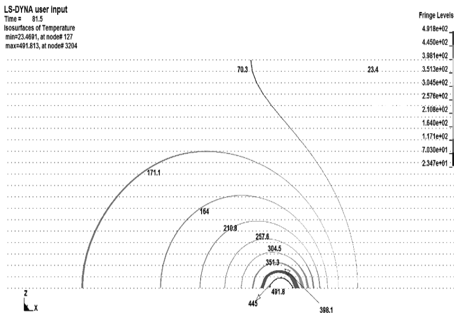
Fig. 3. Isothermal contours through the weld seam after 81.5 seconds at tool travel of 140 mm/min
