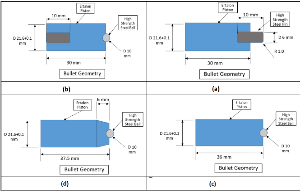
Fig. 2. Drawing of the 4 types of bullets used to hit the target object in the Gas Gan Facility
