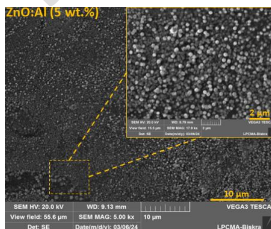
Fig. 8. SEM images Particle size distribution of Al-doped ZnO thin films at different doping concentrations, as determined from SEM analysis.
