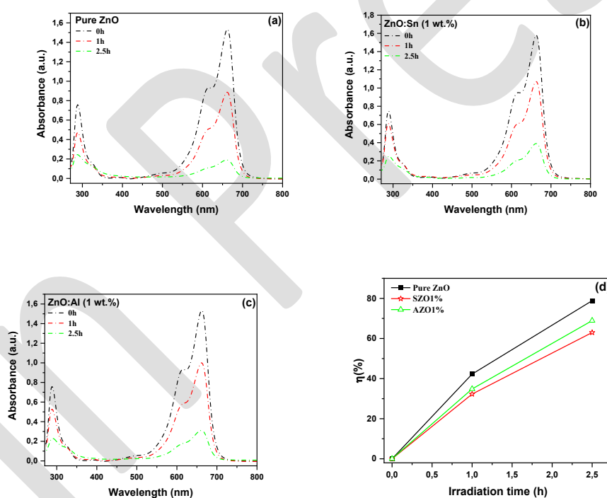
Fig. 12. a–c) UV-Vis absorption spectra of methylene blue (MB) degradation over time under solar irradiation for a) pure ZnO, b) Sn-doped ZnO (1 wt.%), and c) Al-doped ZnO (1 wt.%) thin films. d) Photocatalytic degradation efficiency of MB as a function of irradiation time for pure and doped ZnO thin films.
