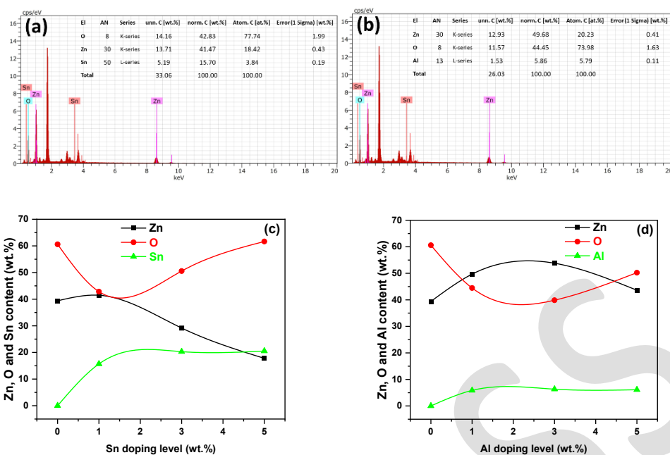
Fig. 6. Elemental composition analysis of ZnO thin films using energy-dispersive X-ray spectroscopy (EDX): a) ZnO:Sn (1 wt.%), b) ZnO:Al (1 wt.%), and c) comparative elemental composition of Sn-doped and d) Al-doped ZnO thin films at different doping concentrations.
