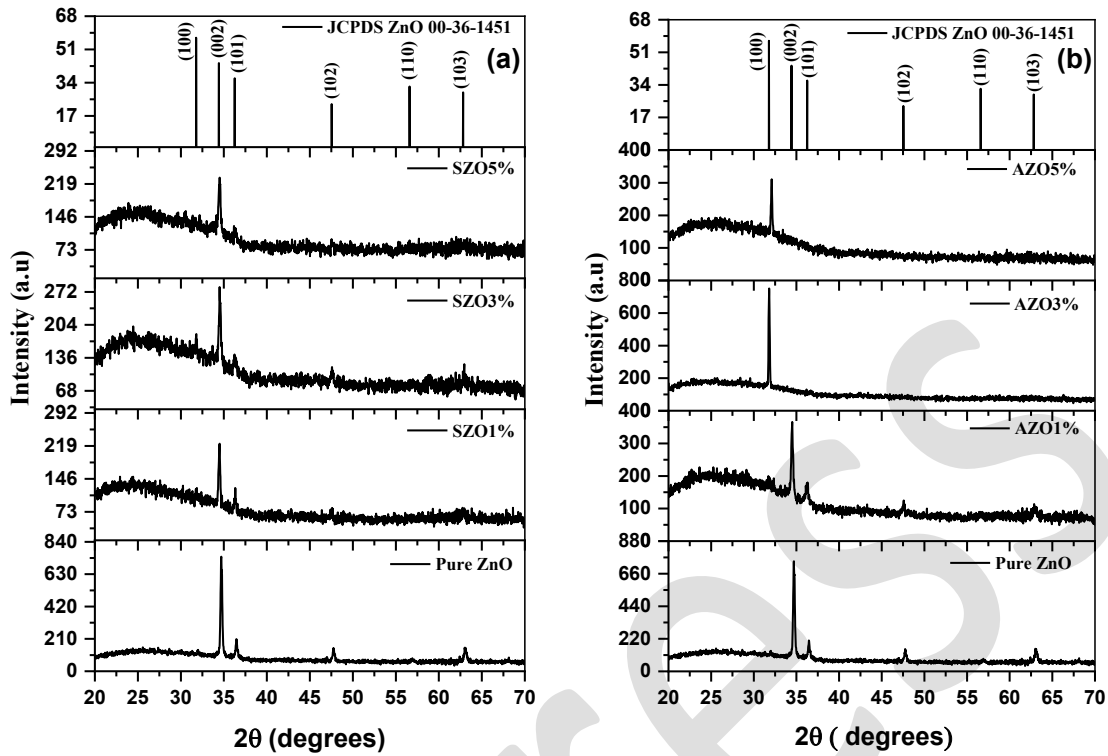
Fig. 3. X-ray diffraction (XRD) patterns of ZnO thin films doped with a) Sn and b) Al, showing characteristic diffraction peaks and changes in crystallinity.
