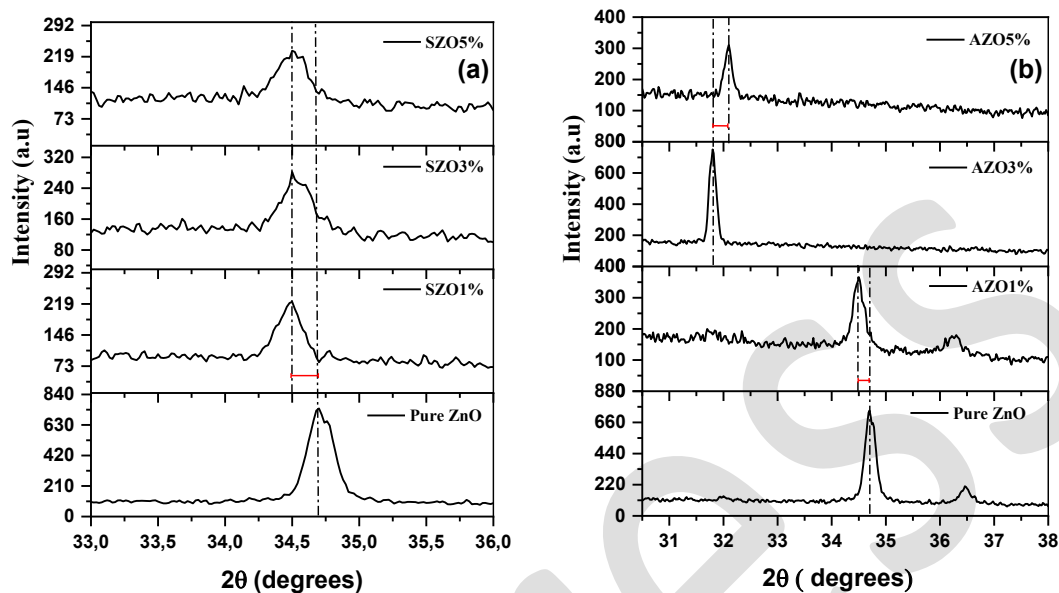
Fig. 4. Enlarged XRD patterns focusing on the (002) diffraction peak for a) Sn-doped ZnO and b) Al-doped ZnO films, highlighting shifts due to doping.
