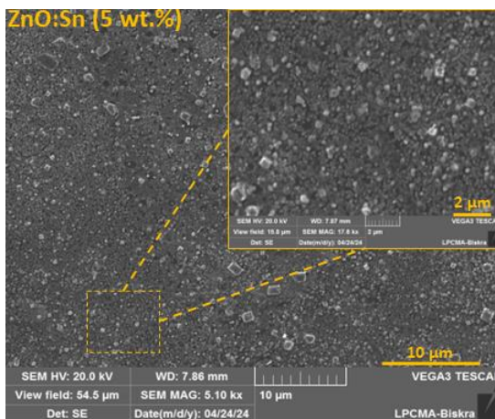
Fig. 7. SEM images and particle size distribution of pure ZnO and Sn-doped ZnO thin films at different doping concentrations, obtained from SEM analysis.
