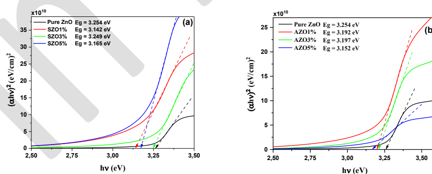
Fig. 10. Tauc plot for bandgap determination of ZnO thin films doped with a) Sn and b) Al, showing variations in optical bandgap energy with doping concentration.
