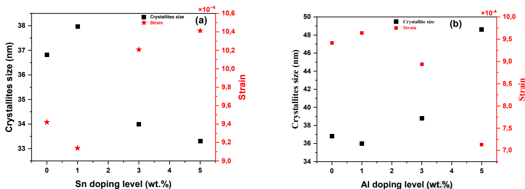
Fig. 5. Effect of a) Sn and b) Al doping concentrations on crystallite size and microstrain in ZnO thin films, calculated using Scherrer's equation.
