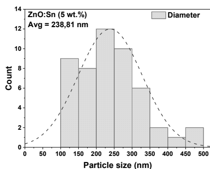
Fig. 7. SEM images and particle size distribution of pure ZnO and Sn-doped ZnO thin films at different doping concentrations, obtained from SEM analysis.
