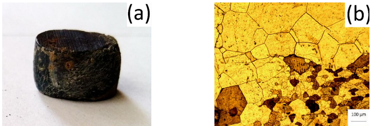
Fig. 8. a) The sample deformed at 900°C and strain rate of 0.1 s -1 and b) corresponding light optical microstructure.
