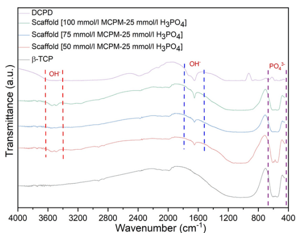
Fig. 9. The FTIR results for the 300\text{--}600\ \mu\text{m} of porous DCPD/ \beta -TCP scaffolds produced after the porous \beta -TCP granules were reacted with three different concentrations of an acidic-CaP solution.
