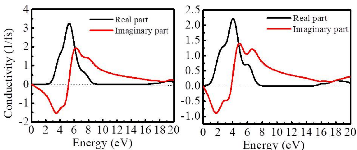
(a) \text{SrTi}_{0.875}\text{Cr}_{0.125}\text{O}_3 (b) \text{SrTi}_{0.750}\text{Cr}_{0.250}\text{O}_3 Fig. 13. The predicted conductivity of doped Cr-SrTiO 3 at Ti sites.
