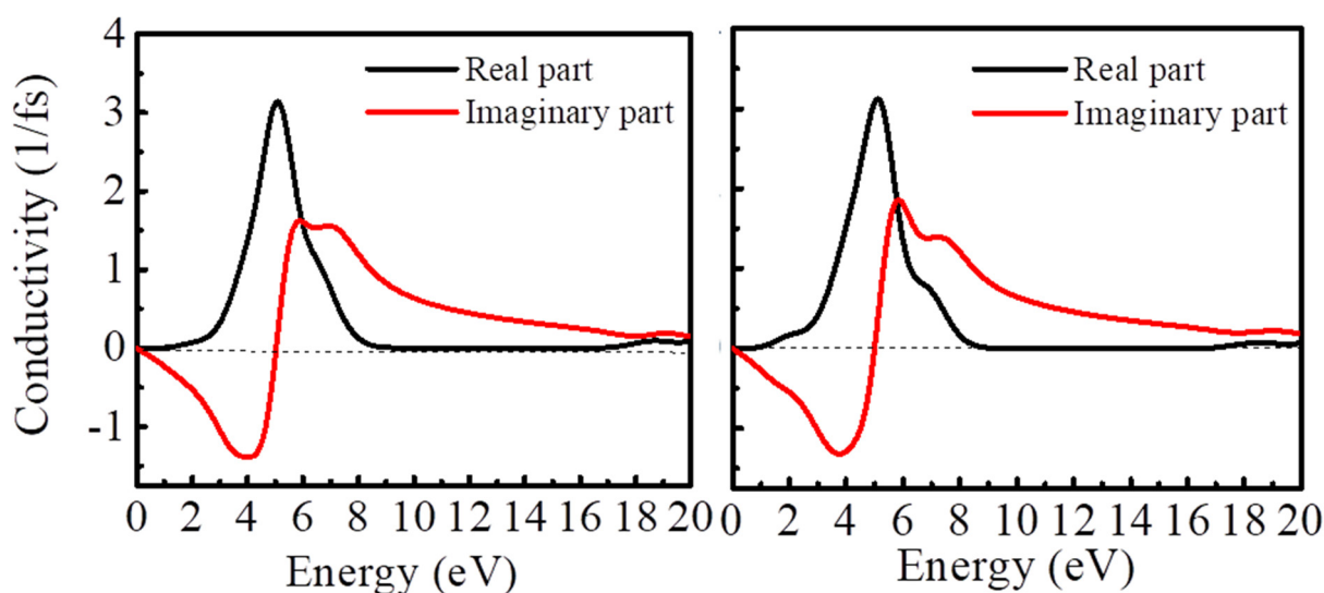
(a) \text{Sr}_{0.875}\text{Cr}_{0.125}\text{TiO}_3 (b) \text{Sr}_{0.750}\text{Cr}_{0.250}\text{TiO}_3 Fig. 14. The predicted conductivity of doped Cr-SrTiO 3 at Sr sites.
