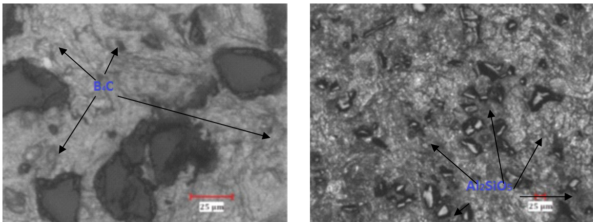
(a) A7, 12% B 4 C, 150 rpm, 12 min
