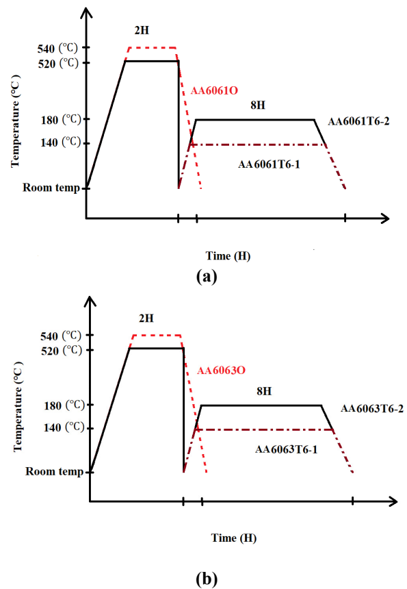
Fig. 1. Schematic of artificial aging heat treatment (T6-1 and T6-2 treatment) and annealing heat treatment (O treatment) for (a) AA6061 and (b) AA6063 aluminum alloys.
