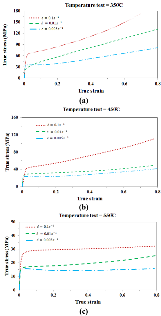
Fig. 6. True stress-true strain curves of AA6061T6-2 for various strain rates at different temperatures of (a) 350°C, (b) 450°C and (c) 550°C.
