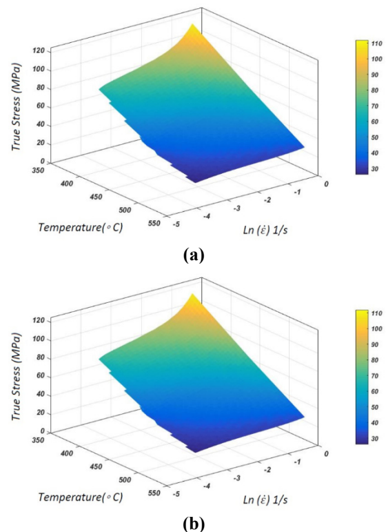
Fig. 8. Representation of flow stress as a function of temperature and strain rate at a strain of 0.8 for (a) AA6061T6-2 and (b) AA6063T6-2.
