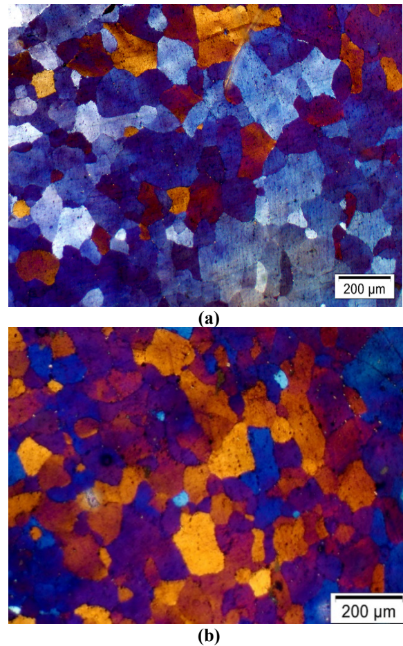
Fig. 2. Optical micrograph of the initial microstructure of (a) AA6061 O and (b) AA6061 T6-2 aluminum alloys.
