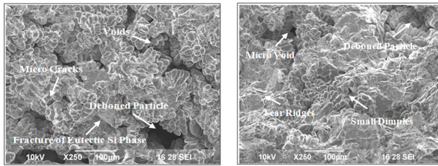
Fig. 13. (a) Fractography of A356-5% TiB 2 /TiC at room temperature. (b) at 300°C temperature.
