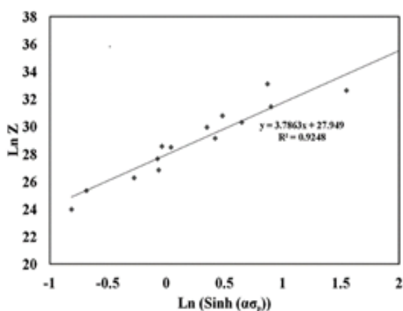
Fig. 9- The relationship between ln Z-ln[sinh(ασ)]
