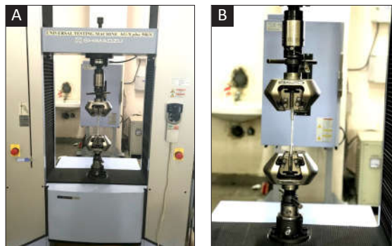
Fig. 4. Tensile Testing Machine (Shimadzu) a) Tensile testing machine (Shimadzu) b) Tensile test specimen loaded in the UTM
