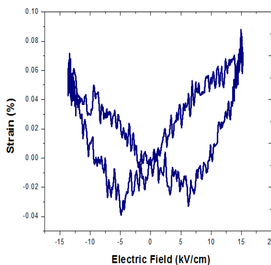
Fig.13. Strain vs. Electric field (S-E) Loops of KNN Ceramics sintered at 1100 °C.
