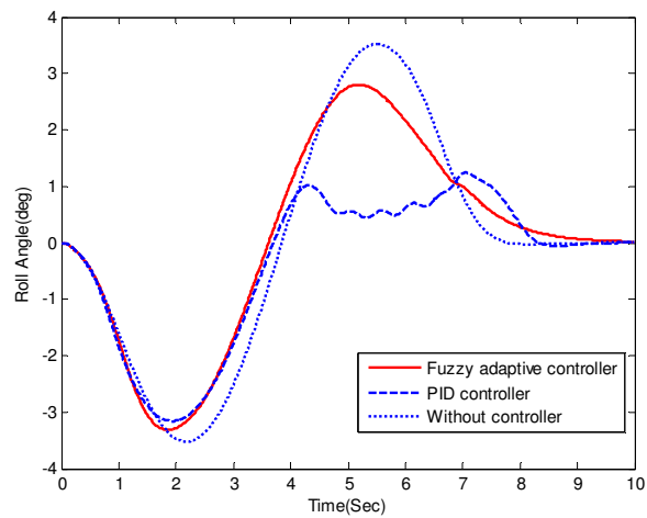
Fig23. Roll angle response for LC manoeuvre
