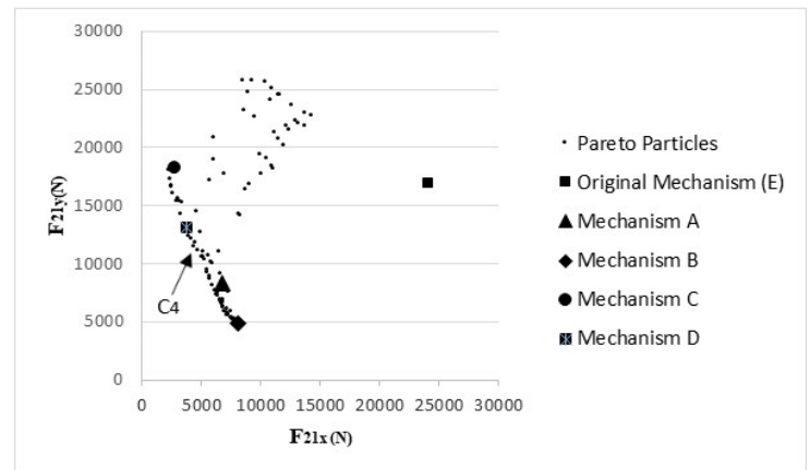
Figure 5: Pareto front of F_{21x} and F_{21y}
