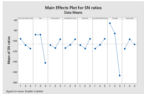
Figure26: First Step Taguchi for Suspension Kinematic Factors
