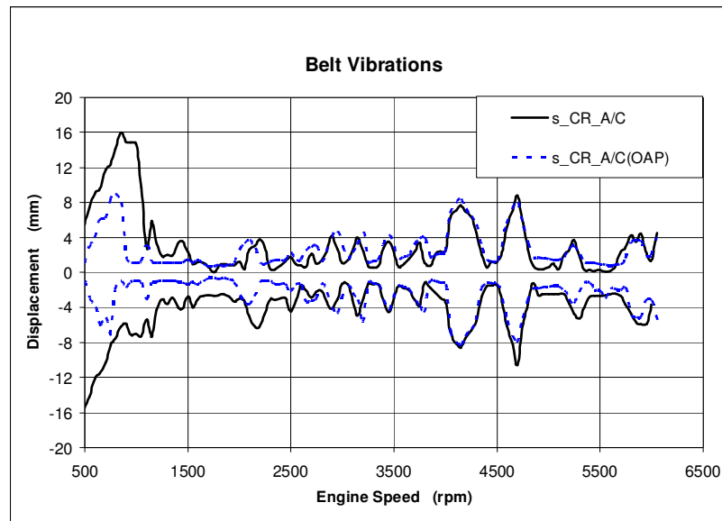
Figure 6. Belt vibration (comparison between result with OAP and without OAP)
