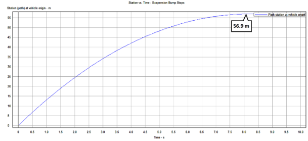
Figure49: Brake Distance m-Time(s) "MAFSMC_ON"
