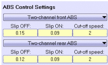
Figure14: Vehicle’s ABS ON/OFF controller in CarSim
