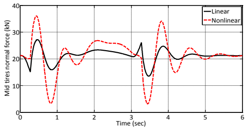
Figure 20. Middle tire normal force
