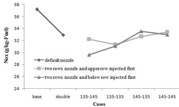
Fig 11. NOx emission
