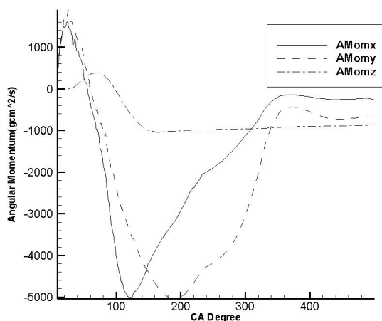
Fig. 13. Predicted angular momentum in three directions with no boost and scavenging
