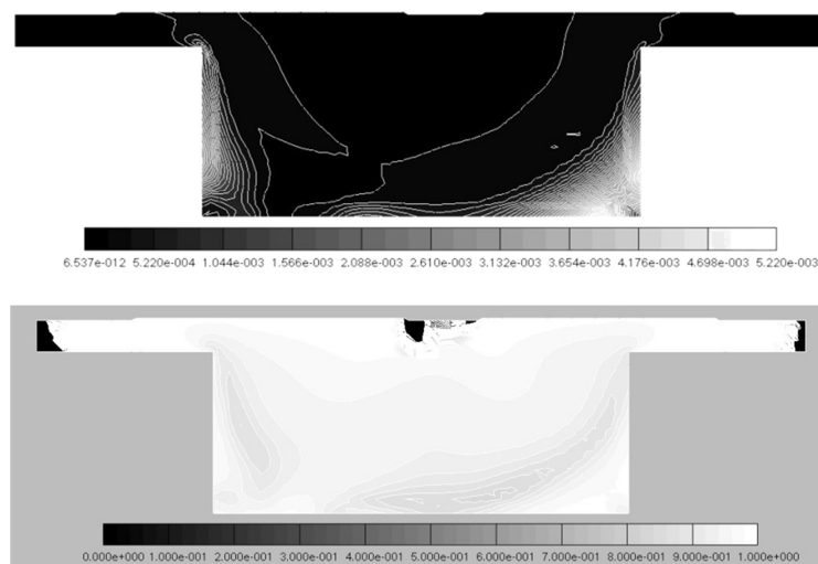
Fig16. Contours of soot mass fraction and flame at 375° CA respectively from top
