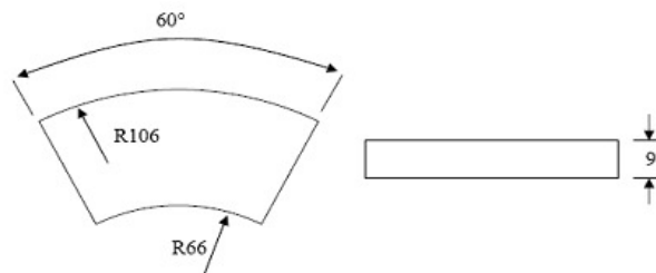
Fig2.the model of disk and pad, and simulation data used in the FE analysis
