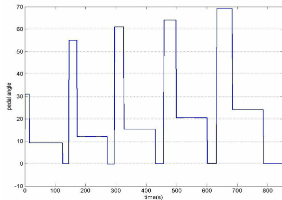
Fig. 11. Input Pedal angle designed for first cycle
